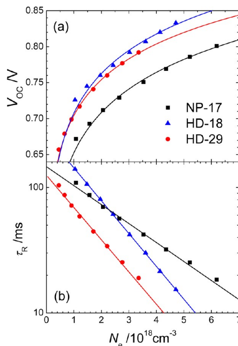
Figure 7. (a) Open-circuit voltage ( V_{OC} ) and (b) electron lifetime ( \tau_R ) as a function of charge density ( N_e ) generated under eight bias white-light irradiations for NP-17, HD-18, and HD-29 devices. HD and NP represent the devices fabricated based on HD1 + HD5 and NP + CCIC films, respectively, with suffixed numeric labels representing total film thickness ( L ).
