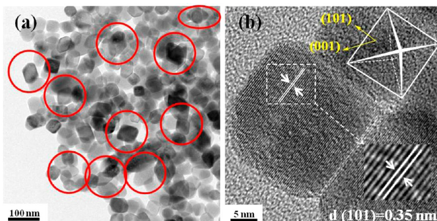
Figure 2. (a) TEM images of HD1 showing the cuboidal morphology of the nanocrystals; the red circles highlight the images with rhombic shapes that represent the formation of octahedron-like nanocrystals. (b) HRTEM image of one specific HD1 single crystal that can be emulated with a 3D octahedral structure with the directions of (101) and (001) planes as indicated; the inset shows the fine structure of the lattice with a distance of 0.35 nm between the (101) facets in the anatase phase.
