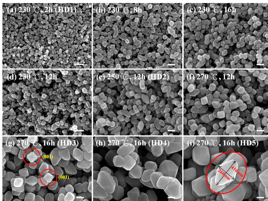
Figure 1. SEM images of TiO 2 nanocrystals in the HD series synthesized at varied hydrothermal conditions: (a) 230 °C and 2 h (HD1), (b) 230 °C and 8 h, (c) 230 °C and 16 h, (d) 230 °C and 12 h, (e) 250 °C and 12 h (HD2), (f) 270 °C and 12 h, (g) 270 °C and 16 h (HD3), (h) repeated hydrothermal treatment using the same sol with HD3 as a seed at 270 °C for 16 h (HD4); the red circles show the (001) facets. (i) Repeated hydrothermal treatment using the same sol with HD4 as a seed at 270 °C for 16 h (HD5); the red circle shows a titania single crystal with a truncated octahedral morphology of an extraordinarily large size. The scale bars indicate 100 nm for each plot.
